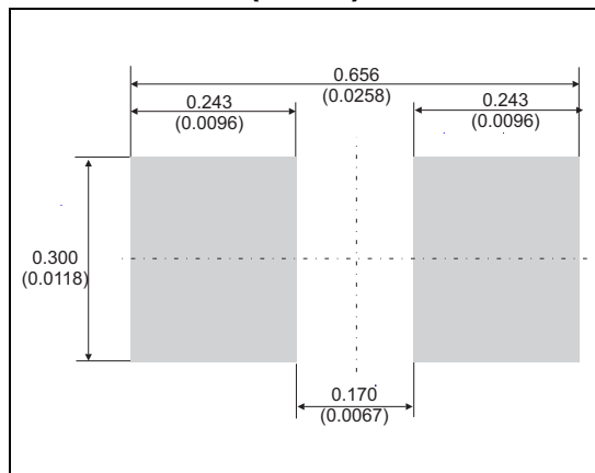
Figure 10. Footprint, dimensions in mm (inches)
