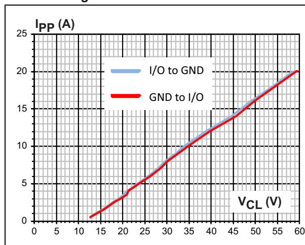
Figure 7. TLP measurements
